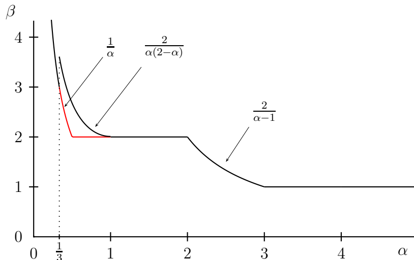
Figure 1: If the random walk R has \alpha finite moments, then the diameter of the resulting n -particle aggregate grows as n^\beta . For \frac{1}{3} < \alpha < 1 our lower and upper bounds for \beta differ, and we believe the lower bound (in red) is correct.
