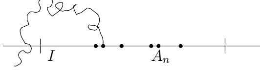
Figure 2: The event that the random walk hits I in A_n .
