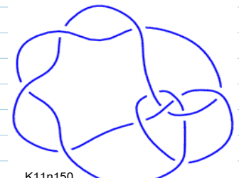
K11n150
