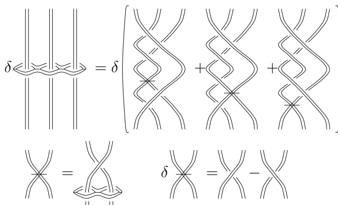
Figure 12. Undoing a Bundle Left Twist one crossing at a time.
