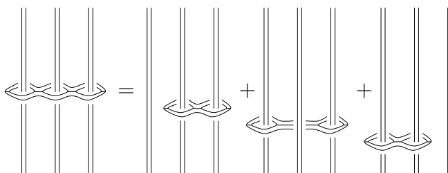
Figure 13. The Total Twist Relation (TTR).
