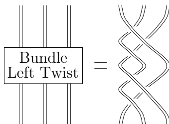
Figure 11. The Bundle Left Twist (BLT) is the same as the Left Twist, only that the strands within each "bundle" are not twisted internally.
