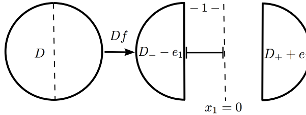
Figure 3. Disconnected targets also produce tears, as do non-convex targets ( \text{spt } \mu^- ).
