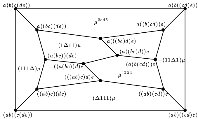
Figure 8. The Stasheff polyhedron — a relation from CA_5
