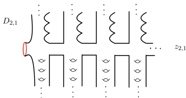
Figure 2 The end z_{2,1} is accumulated by a set of nonplanar ends homeomorphic to \omega^1 and a set of planar ends homeomorphic to \omega^2 . That is, the space of nonplanar ends is homeomorphic to \omega + 1 and the total end space is homeomorphic to \omega^2 + 1 .
