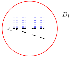
Figure 1 The point z_1 is in the intersection of C_1 and C'_1 . There is a countable set Q_1 of punctures (the blue points) that accumulate to C_1 . Points in C'_1 are not accumulated by punctures except for z_1 .
